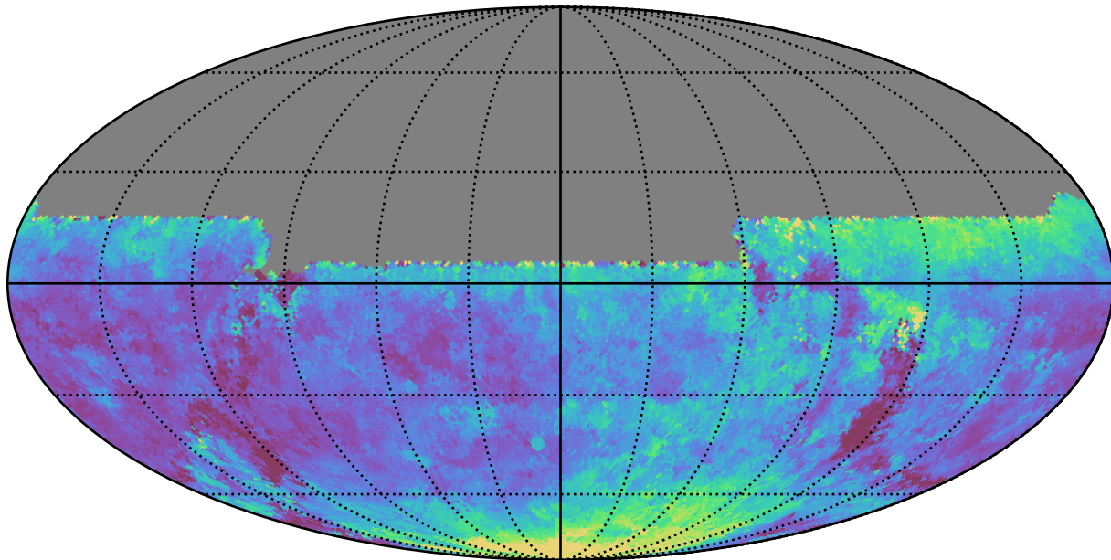
ddf_loaded_fl2_v3.4_10yrs All sky u band: Median seeingEff
