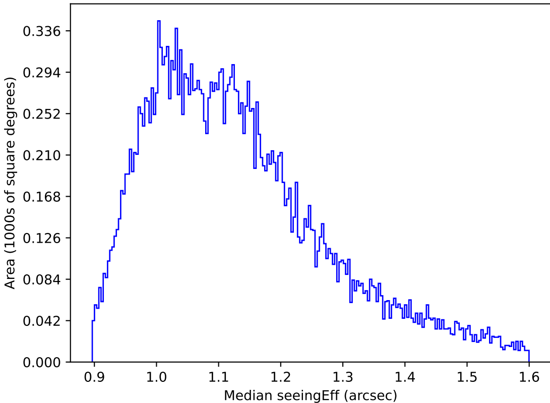
ddf_loaded_fl2_v3.4_10yrs All sky g band: Median seeingEff
