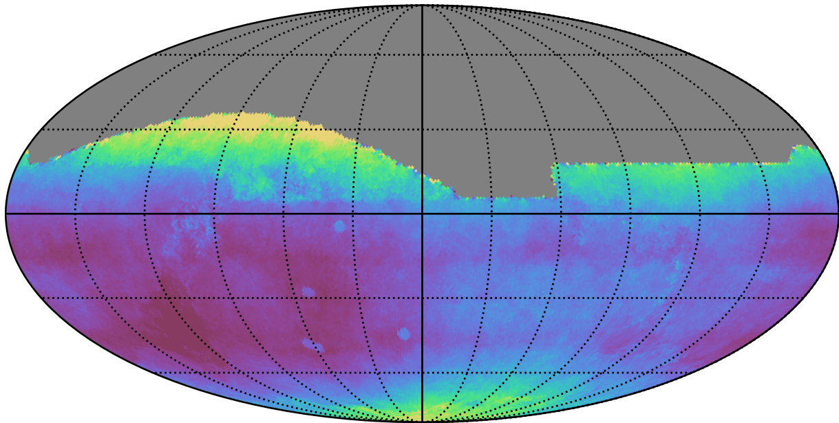
ddf_loaded_fl2_v3.4_10yrs All sky all bands: Median seeingEff
