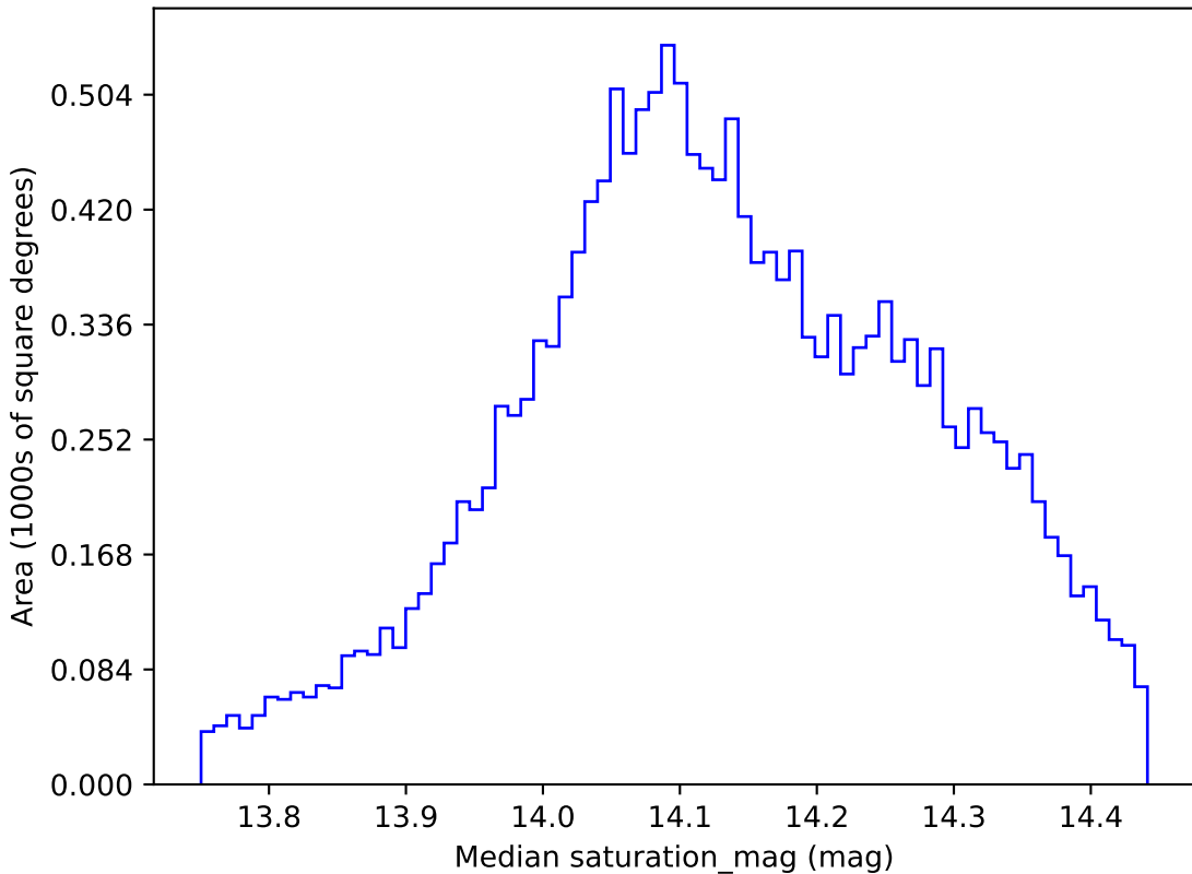
ddf_loaded_fl2_v3.4_10yrs WFD z band: Median saturation_mag
