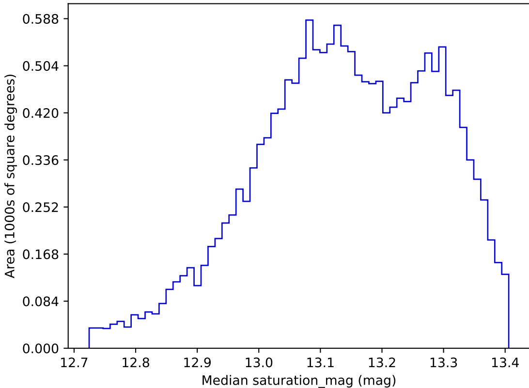
ddf_loaded_fl2_v3.4_10yrs WFD y band: Median saturation_mag
