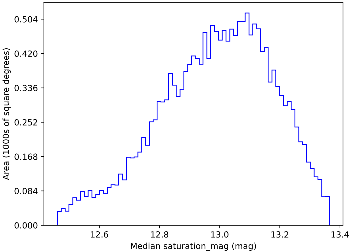
ddf_loaded_fl2_v3.4_10yrs WFD u band: Median saturation_mag
