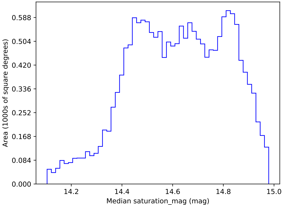
ddf_loaded_fl2_v3.4_10yrs WFD r band: Median saturation_mag
