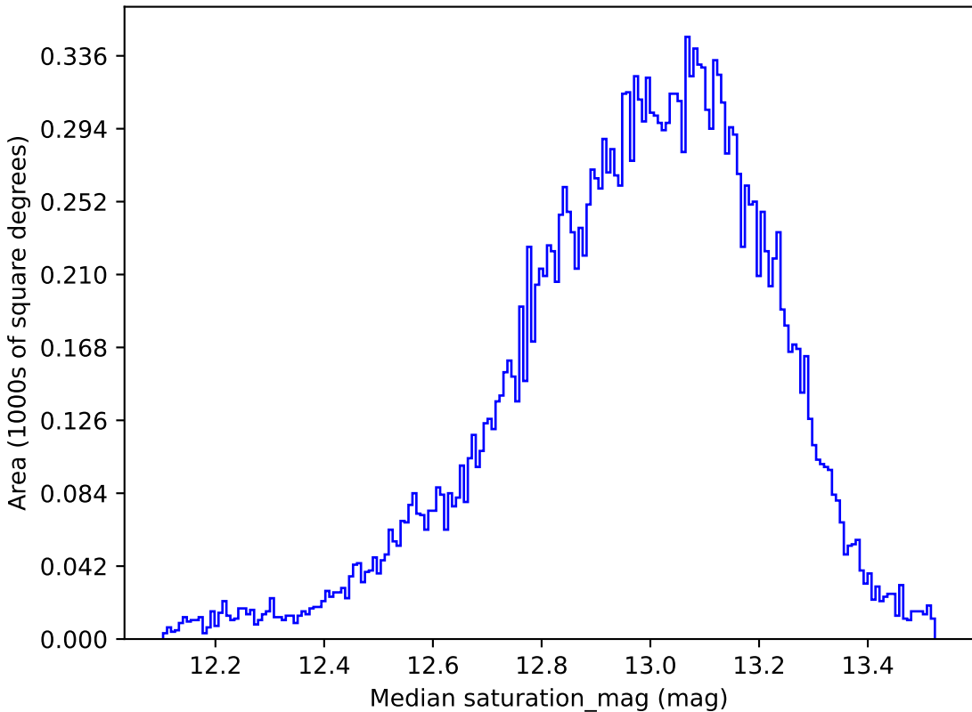
ddf_loaded_fl2_v3.4_10yrs All sky u band: Median saturation_mag
