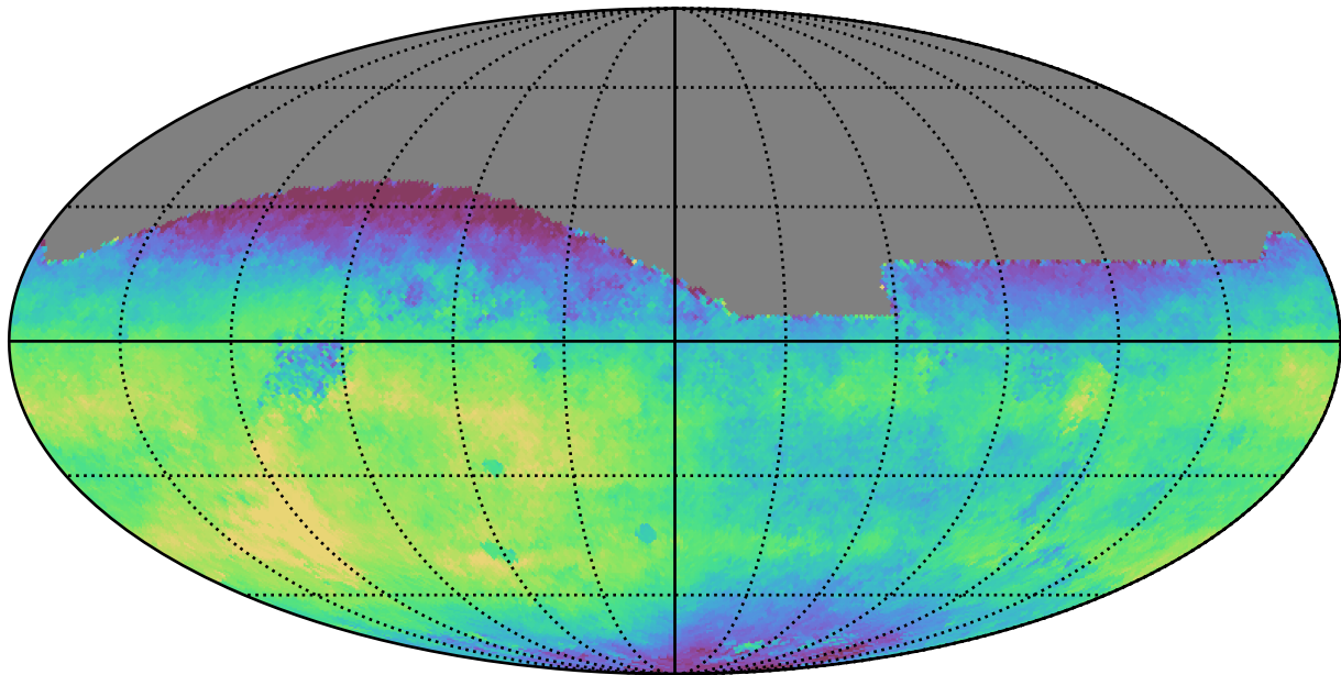
ddf_loaded_fl2_v3.4_10yrs All sky r band: Median saturation_mag
