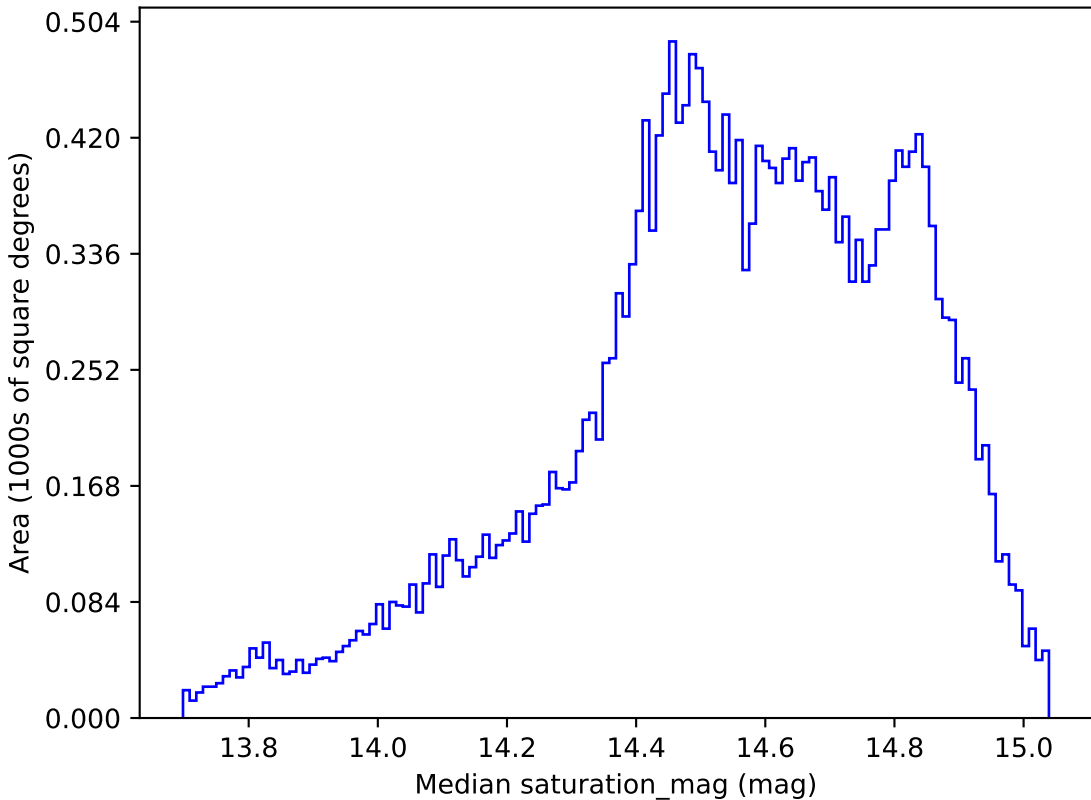
ddf_loaded_fl2_v3.4_10yrs All sky r band: Median saturation_mag
