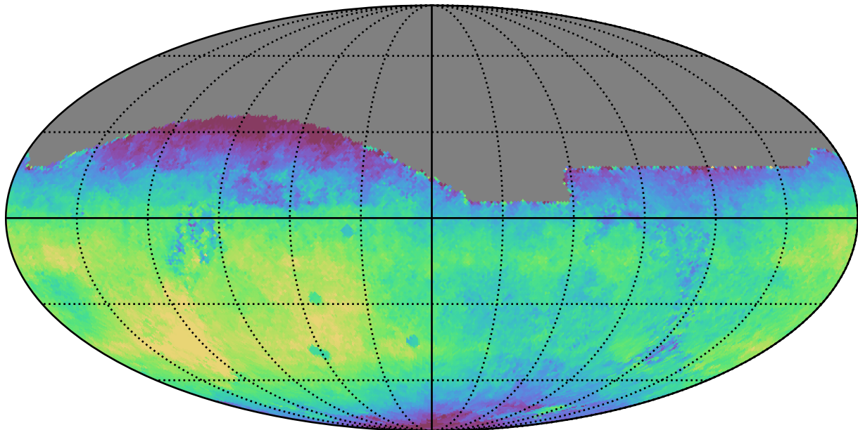
ddf_loaded_fl2_v3.4_10yrs All sky i band: Median saturation_mag
