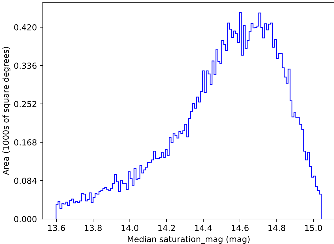
ddf_loaded_fl2_v3.4_10yrs All sky g band: Median saturation_mag
