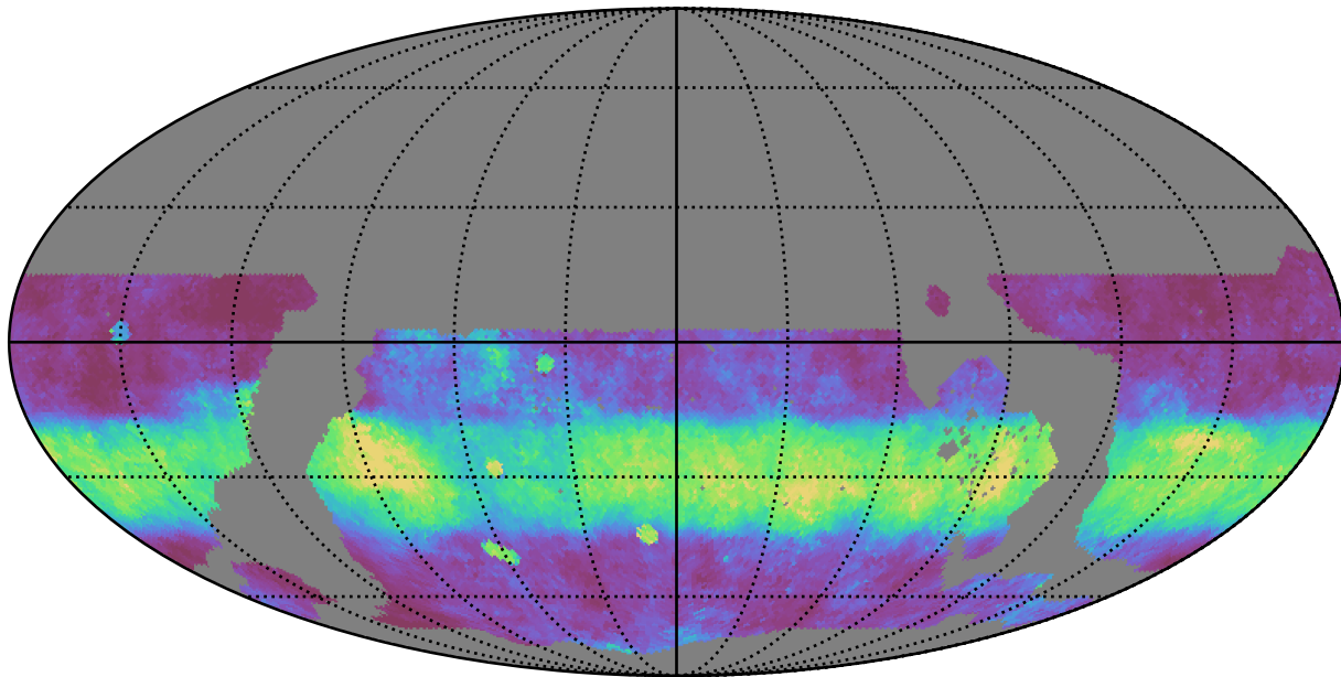
ddf_loaded_fl2_v3.4_10yrs WFD z band: Median normairmass
