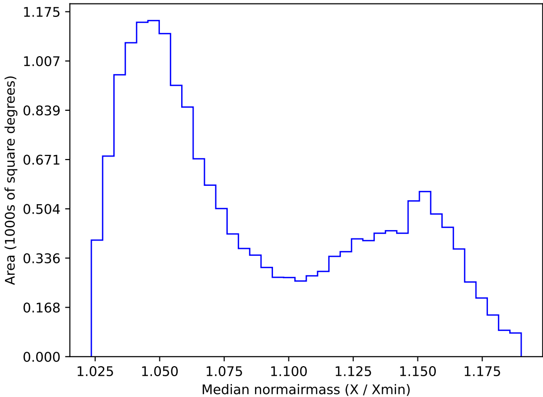
ddf_loaded_fl2_v3.4_10yrs WFD z band: Median normairmass
