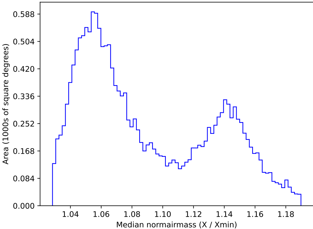
ddf_loaded_fl2_v3.4_10yrs WFD y band: Median normairmass
