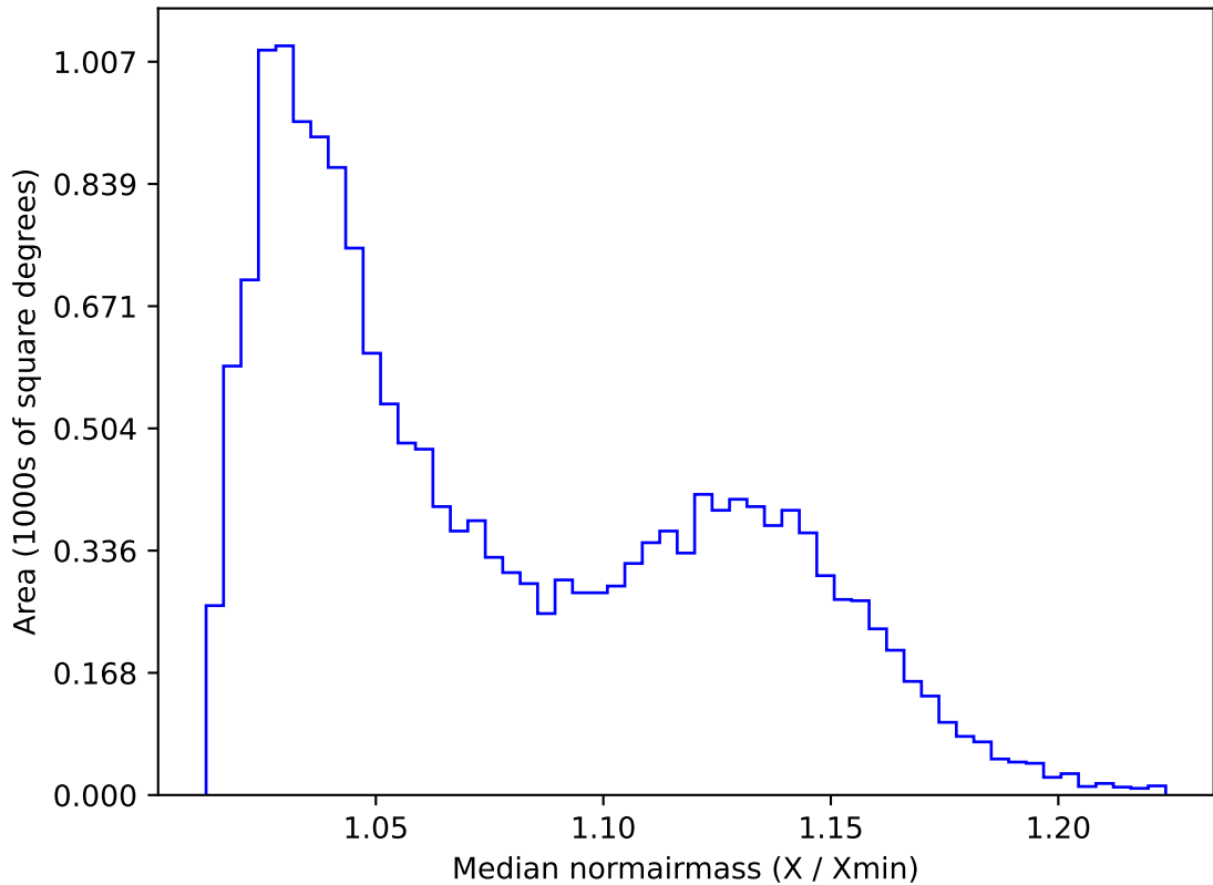
ddf_loaded_fl2_v3.4_10yrs WFD u band: Median normairmass
