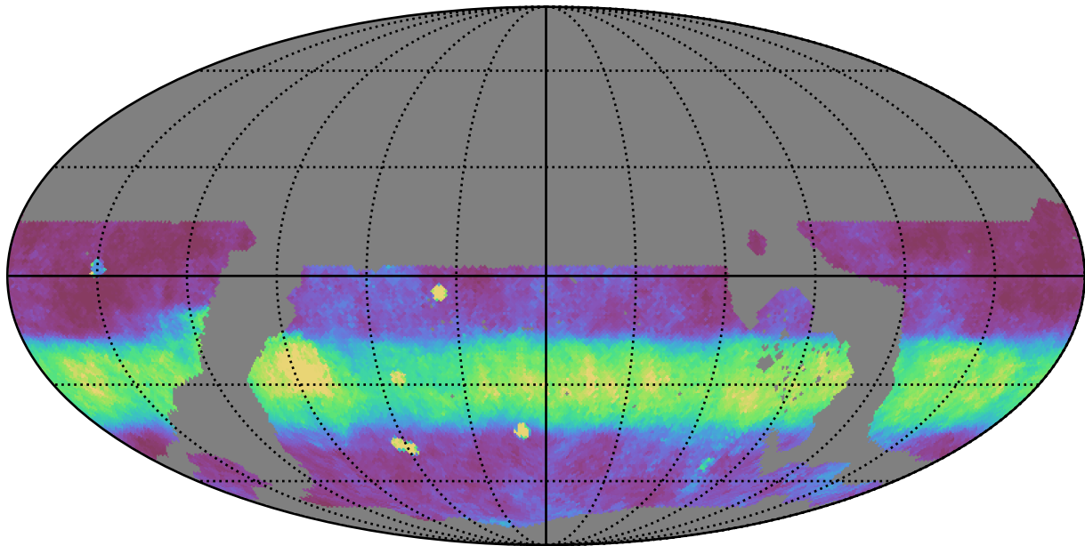
ddf_loaded_fl2_v3.4_10yrs WFD i band: Median normairmass
