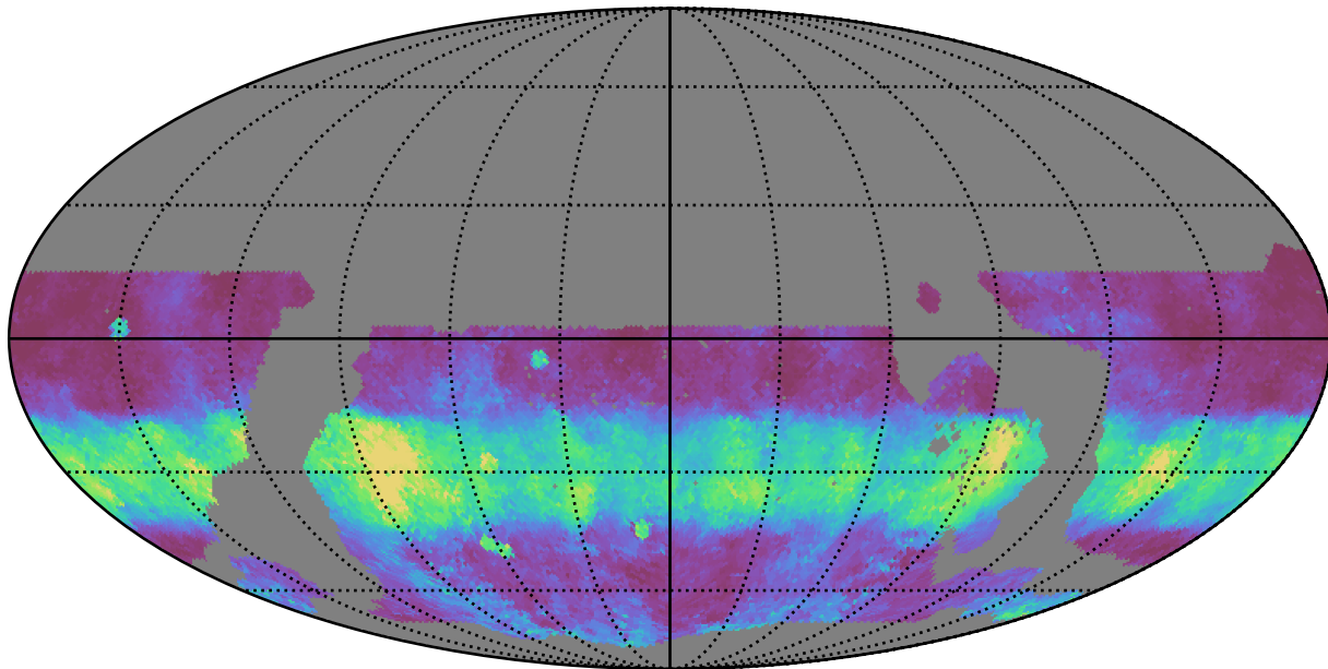
ddf_loaded_fl2_v3.4_10yrs WFD g band: Median normairmass
