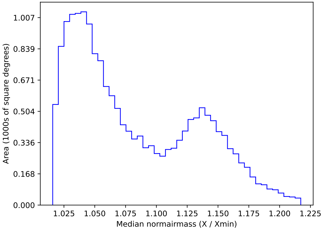
ddf_loaded_fl2_v3.4_10yrs WFD g band: Median normairmass
