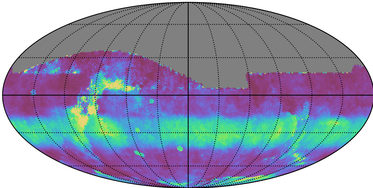
ddf_loaded_fl2_v3.4_10yrs All sky z band: Median normairmass
