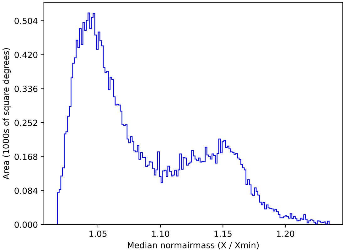
ddf_loaded_fl2_v3.4_10yrs All sky z band: Median normairmass
