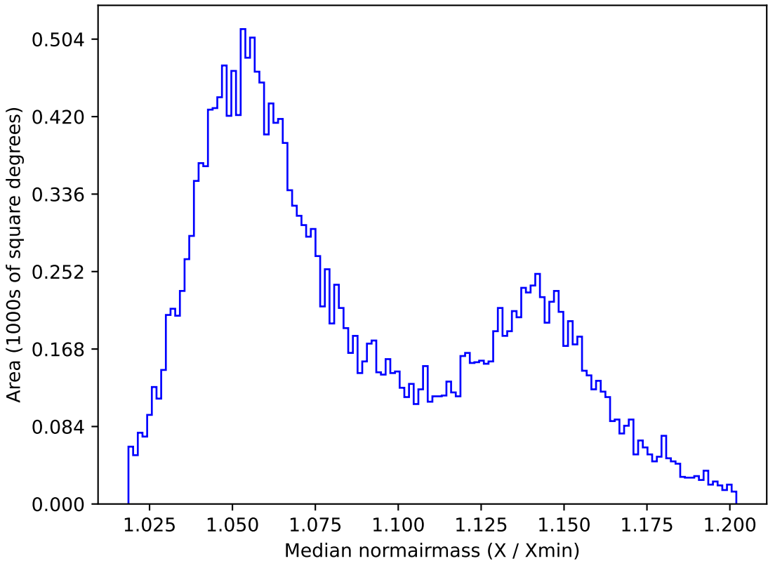
ddf_loaded_fl2_v3.4_10yrs All sky y band: Median normairmass
