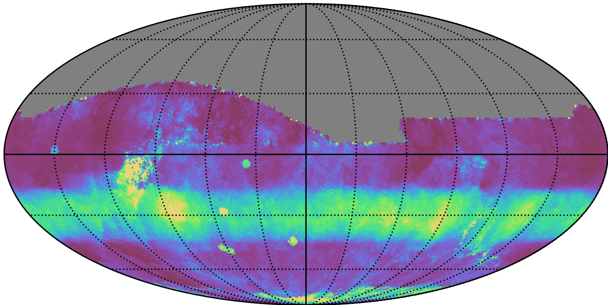
ddf_loaded_fl2_v3.4_10yrs All sky r band: Median normairmass
