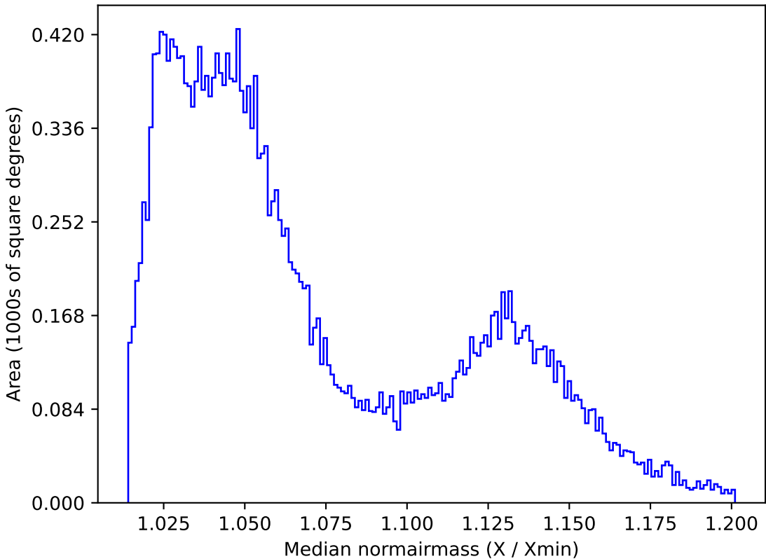
ddf_loaded_fl2_v3.4_10yrs All sky r band: Median normairmass
