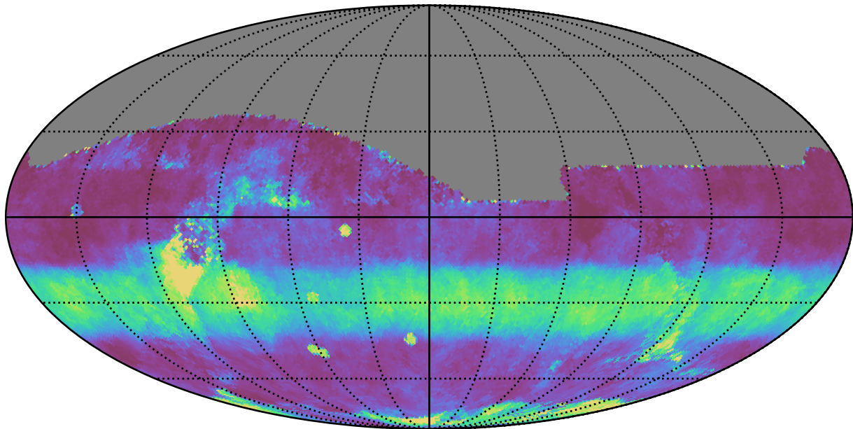
ddf_loaded_fl2_v3.4_10yrs All sky i band: Median normairmass
