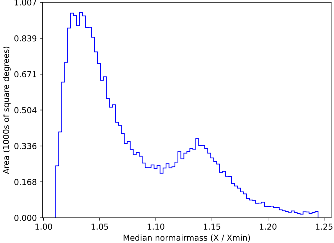
ddf_loaded_fl2_v3.4_10yrs All sky g band: Median normairmass
