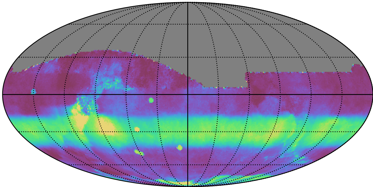
ddf_loaded_fl2_v3.4_10yrs All sky all bands: Median normairmass
