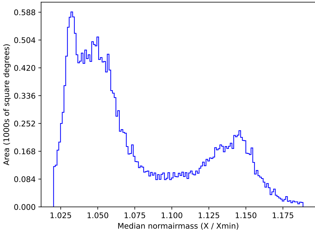
ddf_loaded_fl2_v3.4_10yrs All sky all bands: Median normairmass
