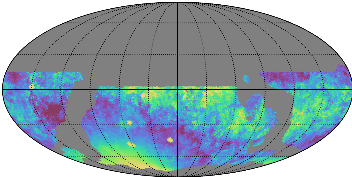
ddf_loaded_fl2_v3.4_10yrs WFD z band: Median moonDistance
