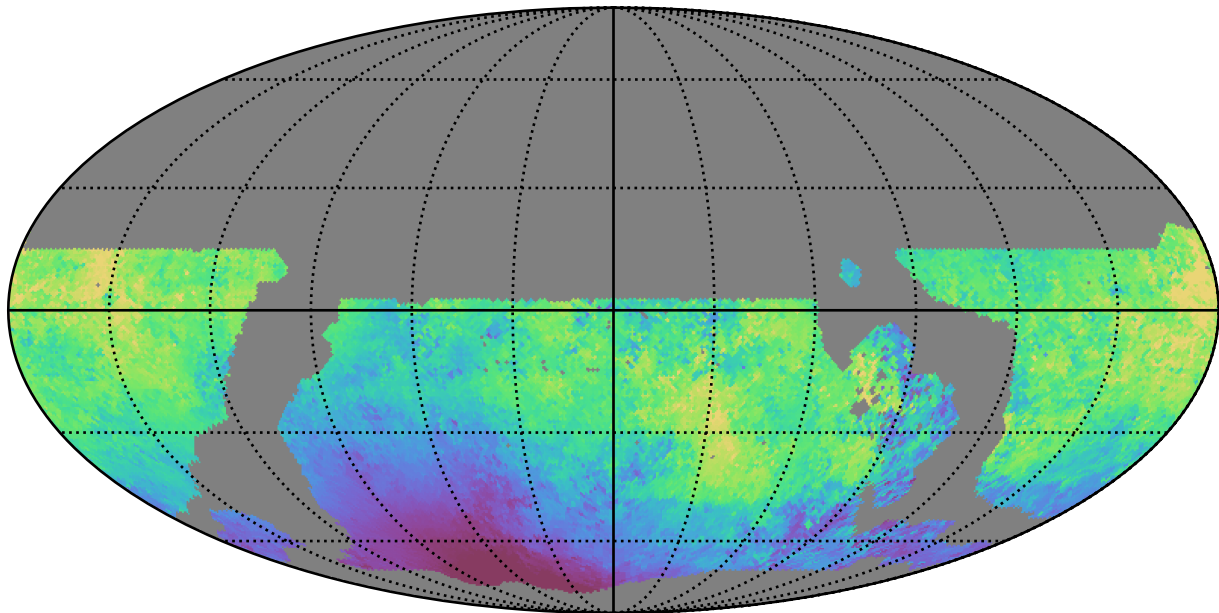
ddf_loaded_fl2_v3.4_10yrs WFD u band: Median moonDistance
