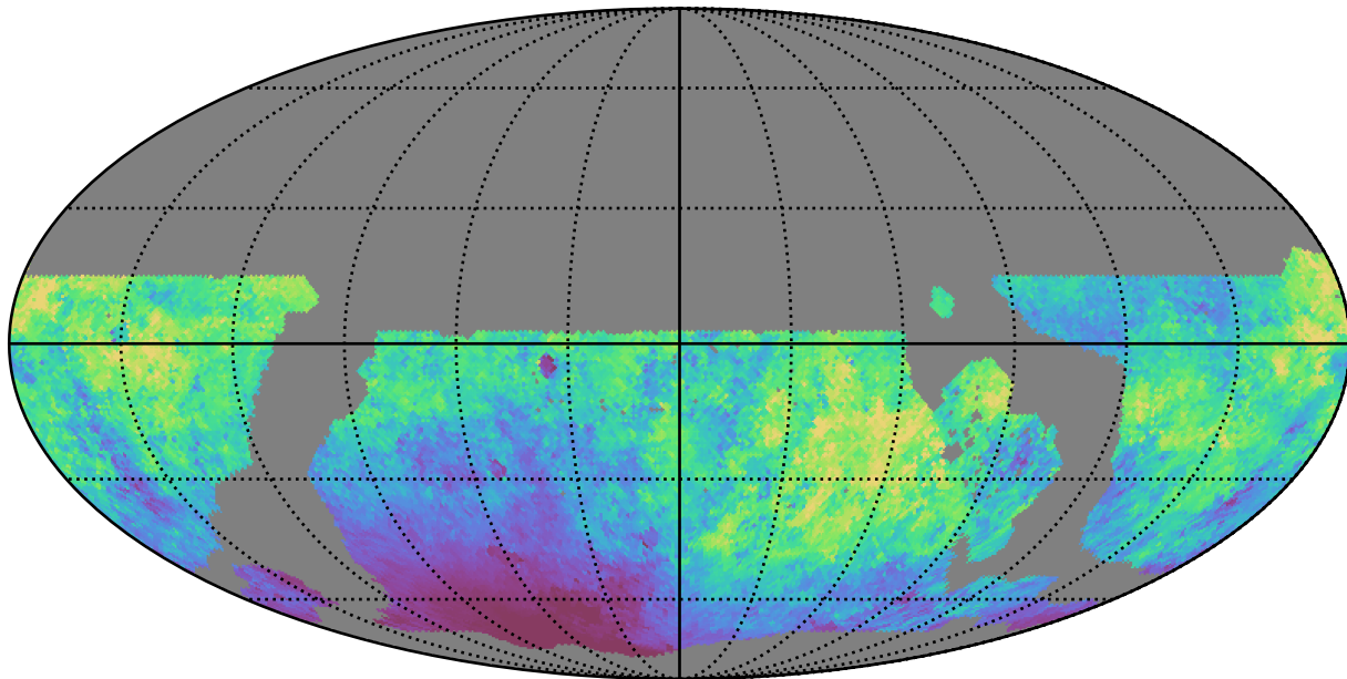
ddf_loaded_fl2_v3.4_10yrs WFD r band: Median moonDistance
