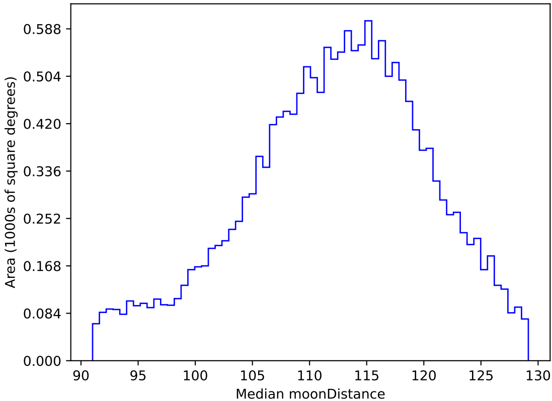
ddf_loaded_fl2_v3.4_10yrs WFD r band: Median moonDistance
