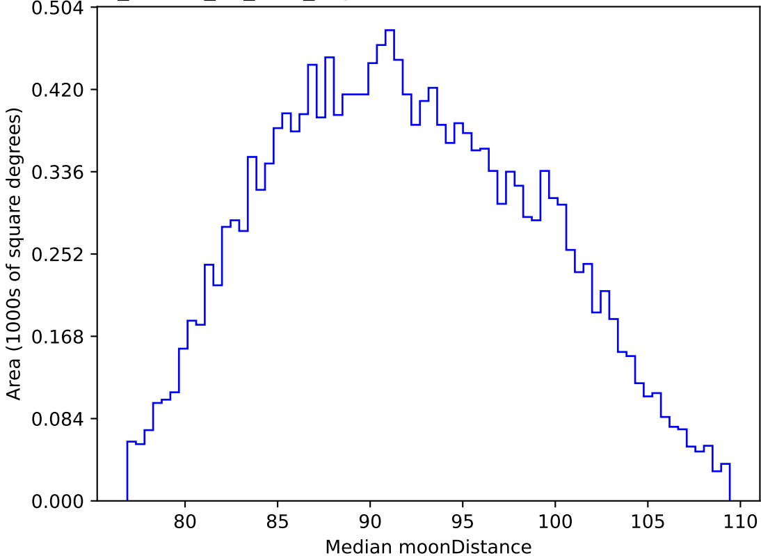
ddf_loaded_fl2_v3.4_10yrs WFD i band: Median moonDistance
