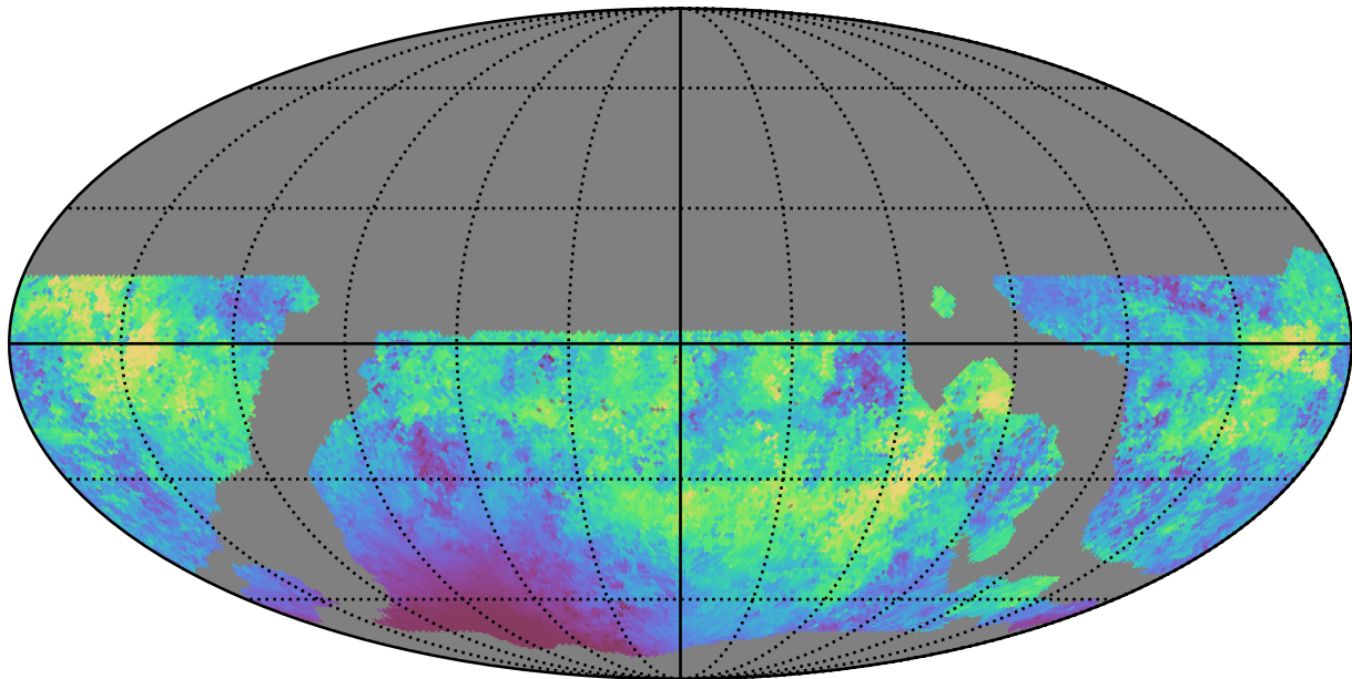
ddf_loaded_fl2_v3.4_10yrs WFD g band: Median moonDistance
