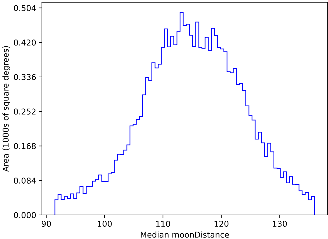
ddf_loaded_fl2_v3.4_10yrs WFD g band: Median moonDistance
