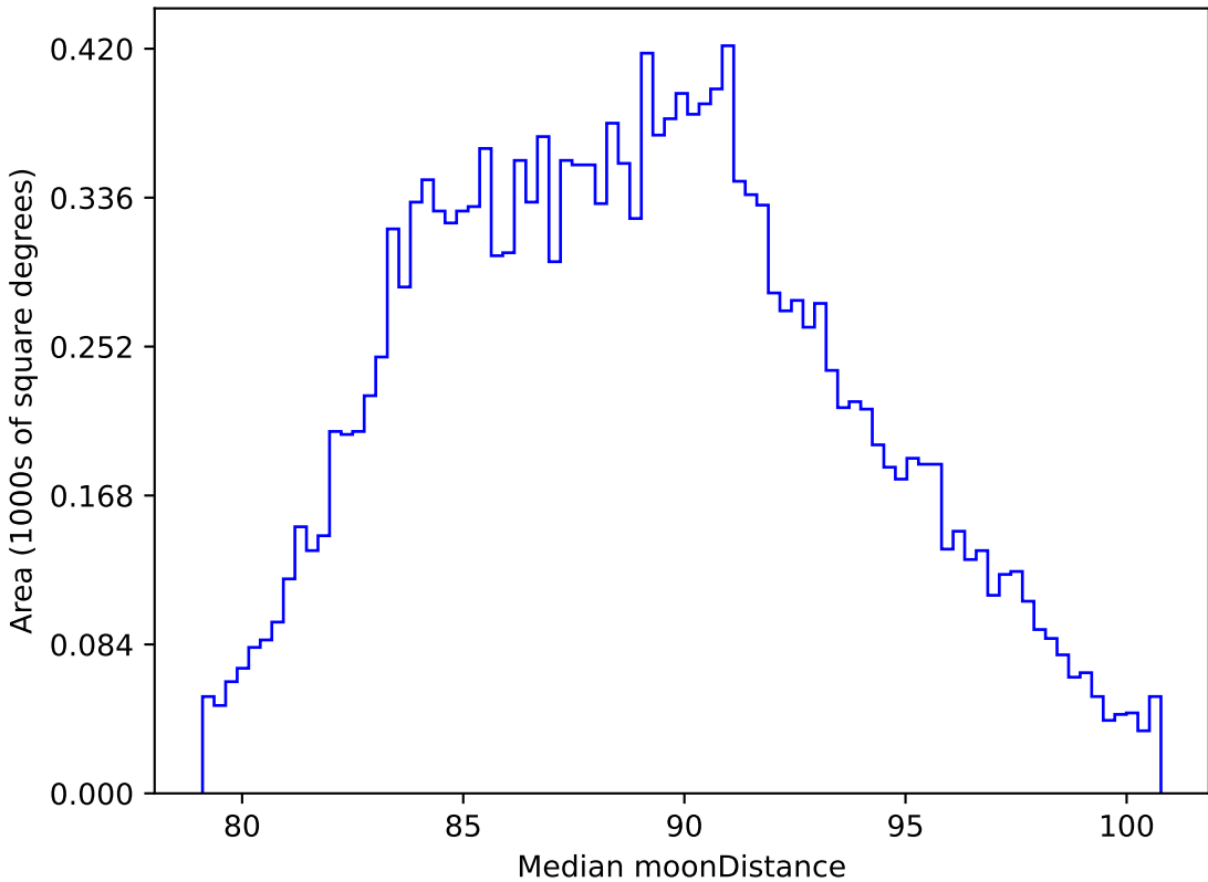
ddf_loaded_fl2_v3.4_10yrs WFD all bands: Median moonDistance
