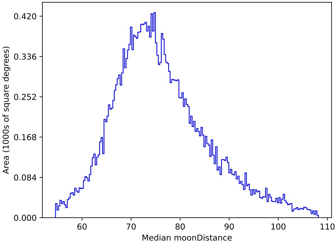
ddf_loaded_fl2_v3.4_10yrs All sky z band: Median moonDistance
