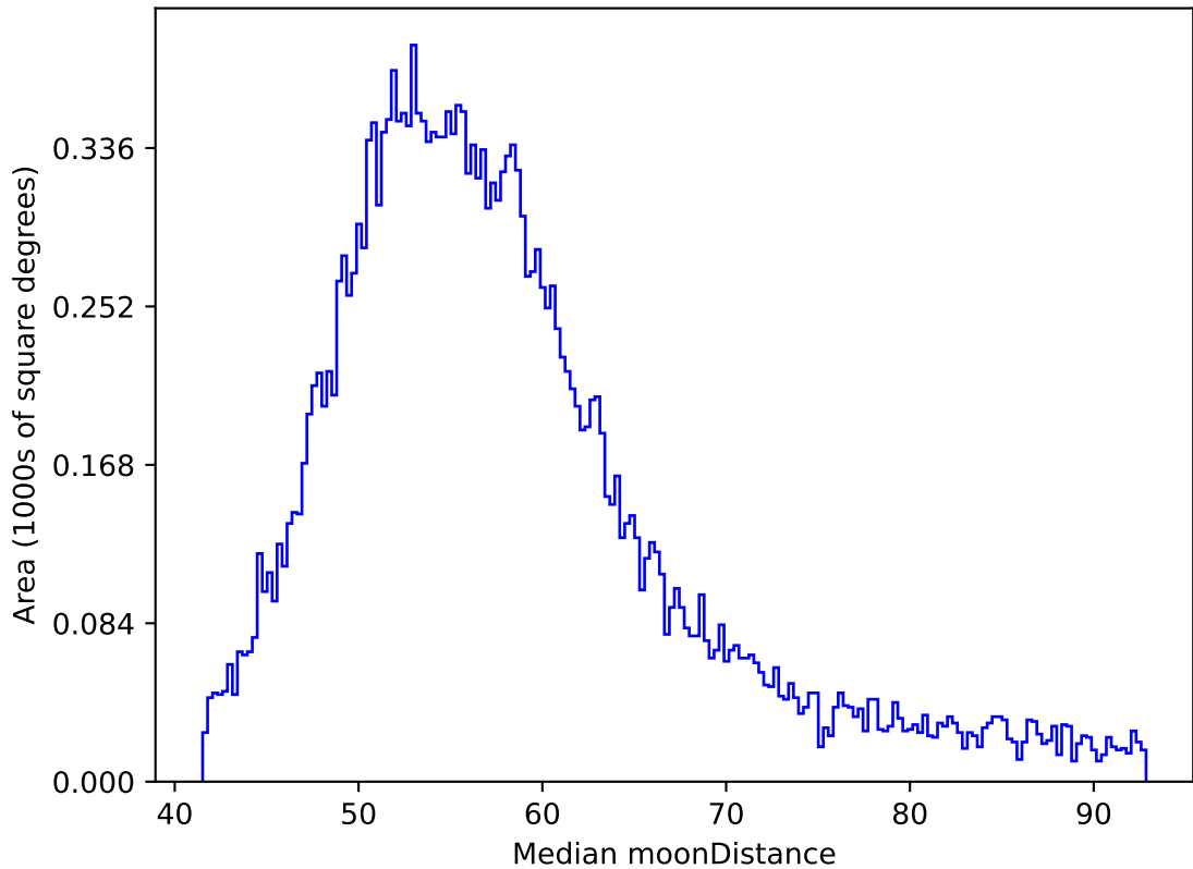
ddf_loaded_fl2_v3.4_10yrs All sky y band: Median moonDistance
