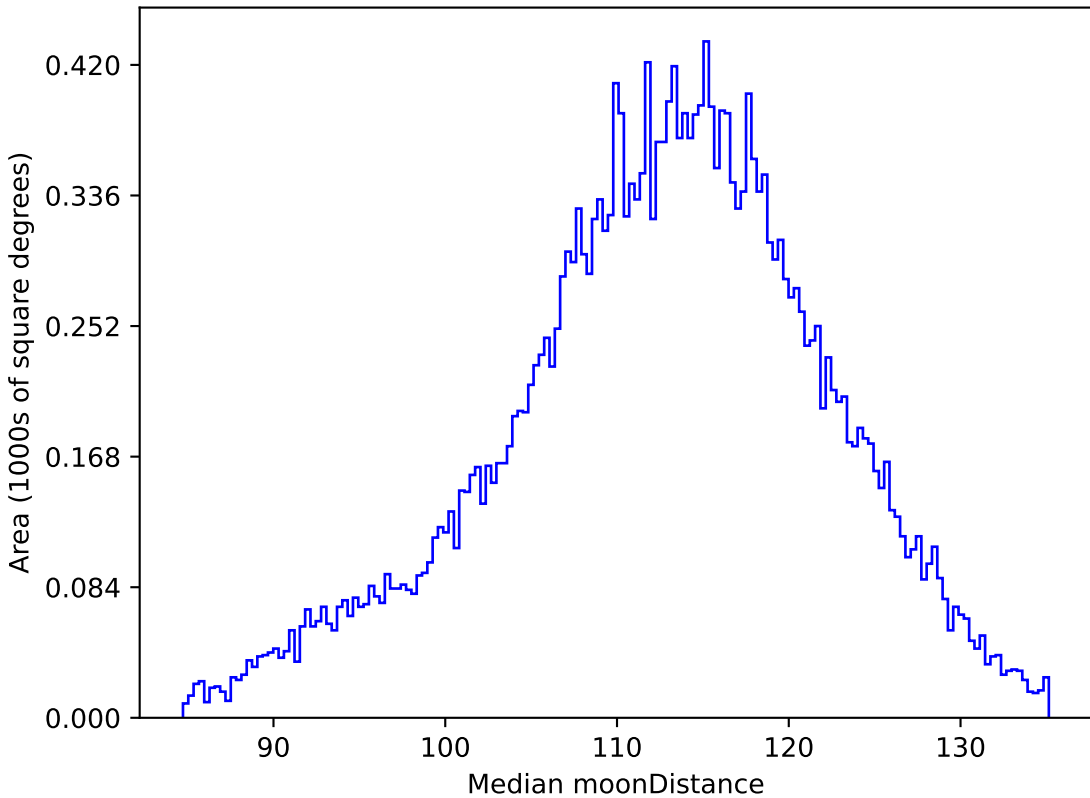
ddf_loaded_fl2_v3.4_10yrs All sky r band: Median moonDistance
