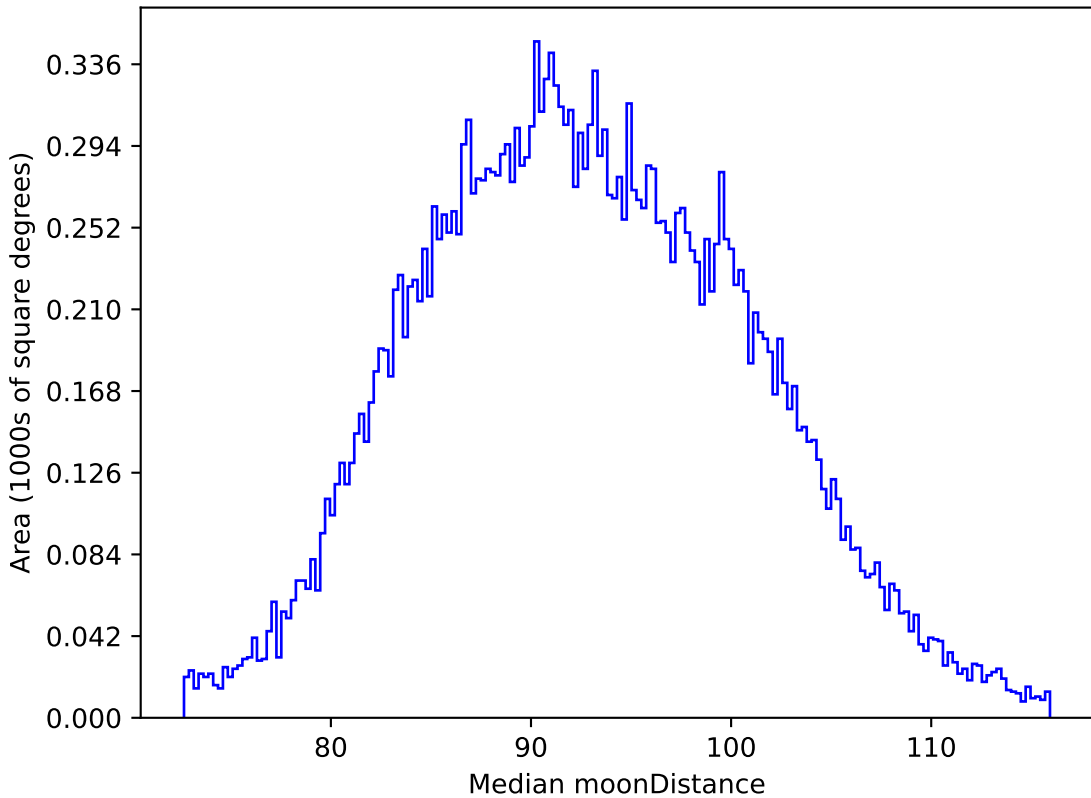
ddf_loaded_fl2_v3.4_10yrs All sky i band: Median moonDistance
