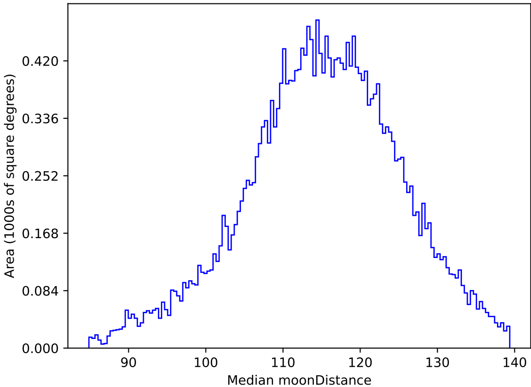
ddf_loaded_fl2_v3.4_10yrs All sky g band: Median moonDistance
