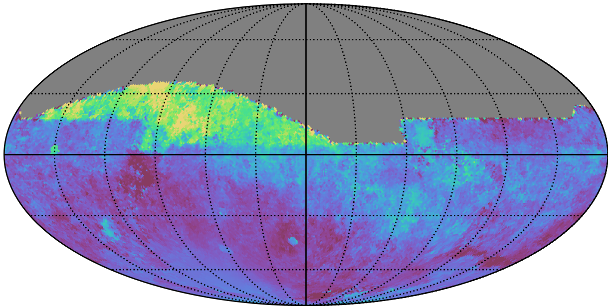
ddf_loaded_fl2_v3.4_10yrs All sky all bands: Median moonDistance
