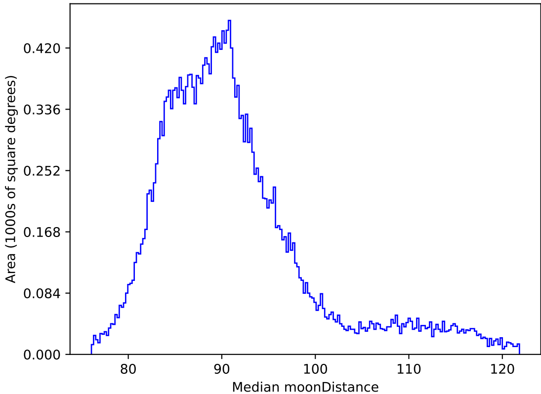
ddf_loaded_fl2_v3.4_10yrs All sky all bands: Median moonDistance
