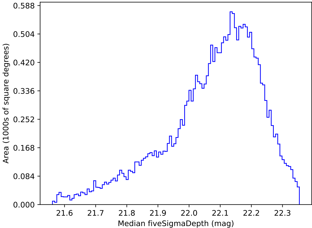
ddf_loaded_fl2_v3.4_10yrs Yr 1 y band: Median fiveSigmaDepth
