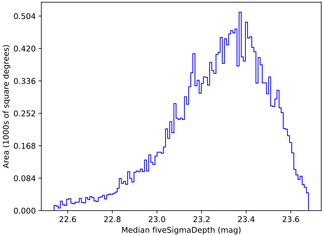
ddf_loaded_fl2_v3.4_10yrs Yr 1 u band: Median fiveSigmaDepth
