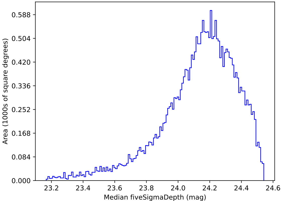
ddf_loaded_fl2_v3.4_10yrs Yr 1 r band: Median fiveSigmaDepth
