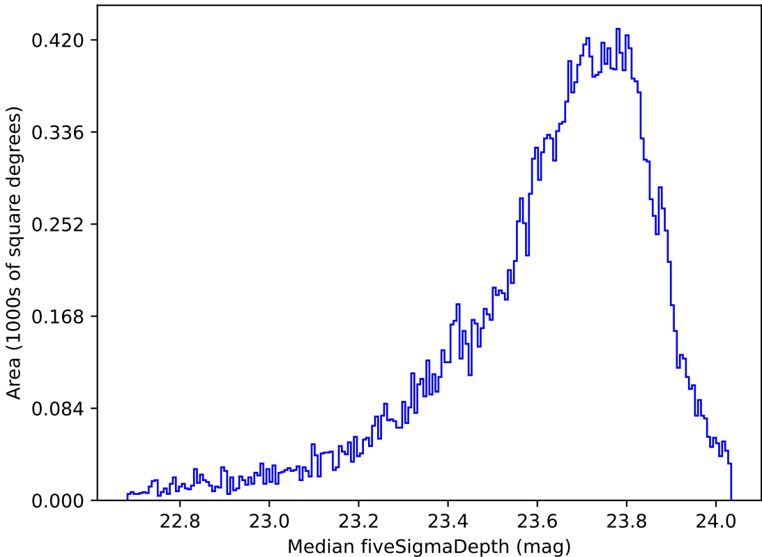
ddf_loaded_fl2_v3.4_10yrs Yr 1 i band: Median fiveSigmaDepth
