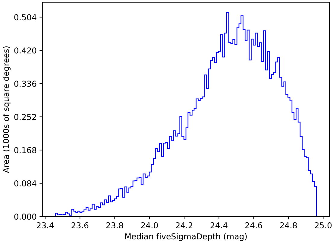
ddf_loaded_fl2_v3.4_10yrs Yr 1 g band: Median fiveSigmaDepth
