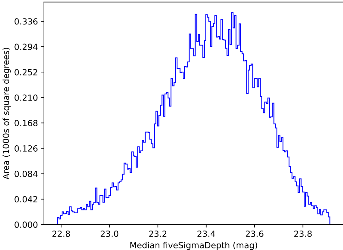
ddf_loaded_fl2_v3.4_10yrs Yr 1 all bands: Median fiveSigmaDepth
