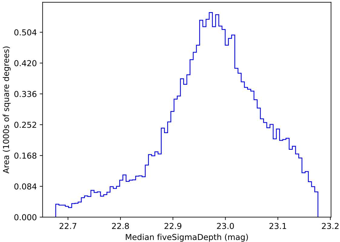
ddf_loaded_fl2_v3.4_10yrs WFD z band: Median fiveSigmaDepth
